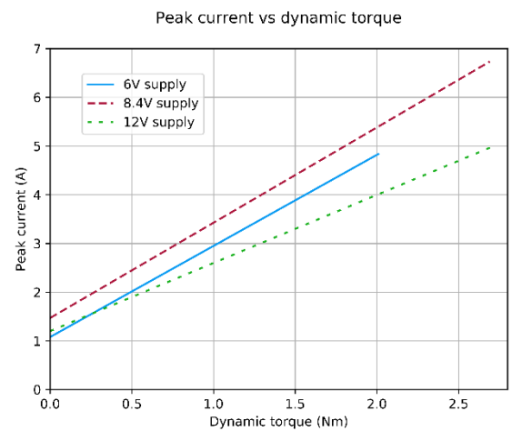
Figure 5: Servo peak current vs dynamic torque. 'Peak current' is measured when the servo is slewing to a new position under load.
