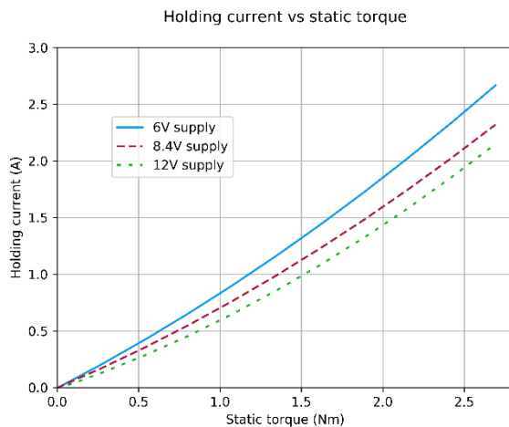
Figure 6: Servo holding current vs static torque. 'Holding current' is measured when the servo is holding position under load.
