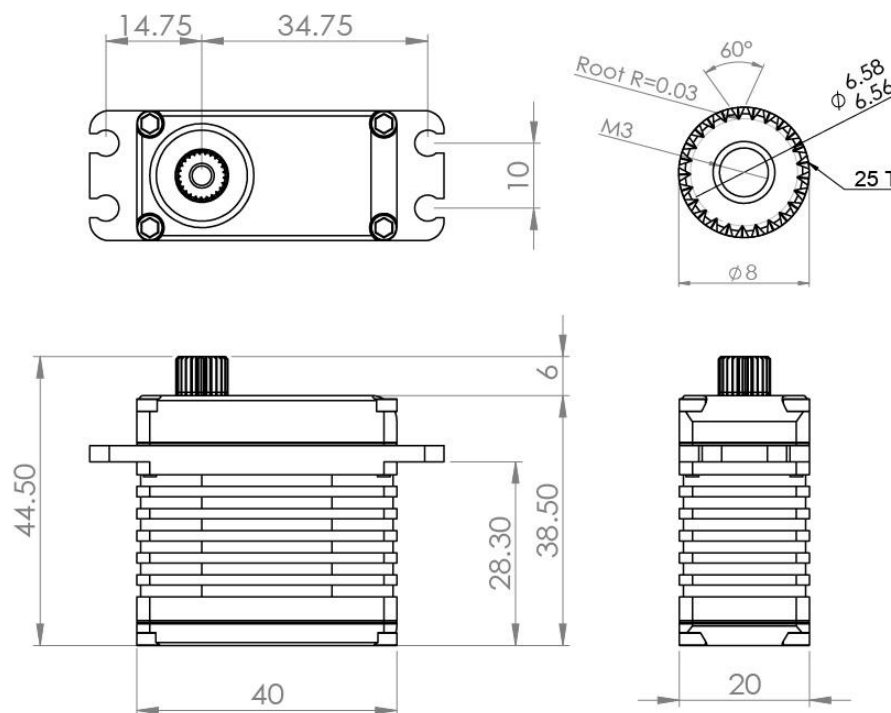
Figure 1: CBS-20 dimensions.
