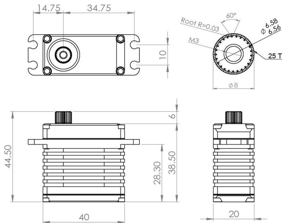
Figure 1: CBS-20 dimensions.
