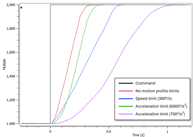
Figure 2: Servo position step response with different motion control profiles.
