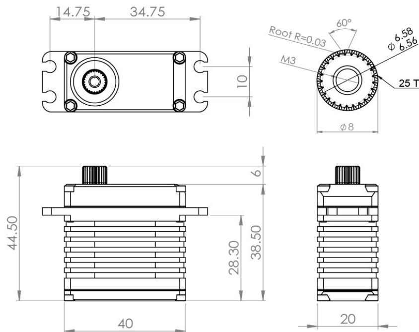
Figure 1: CBS-20 dimensions.
